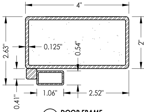
35 DOOR FRAME Foam filled
