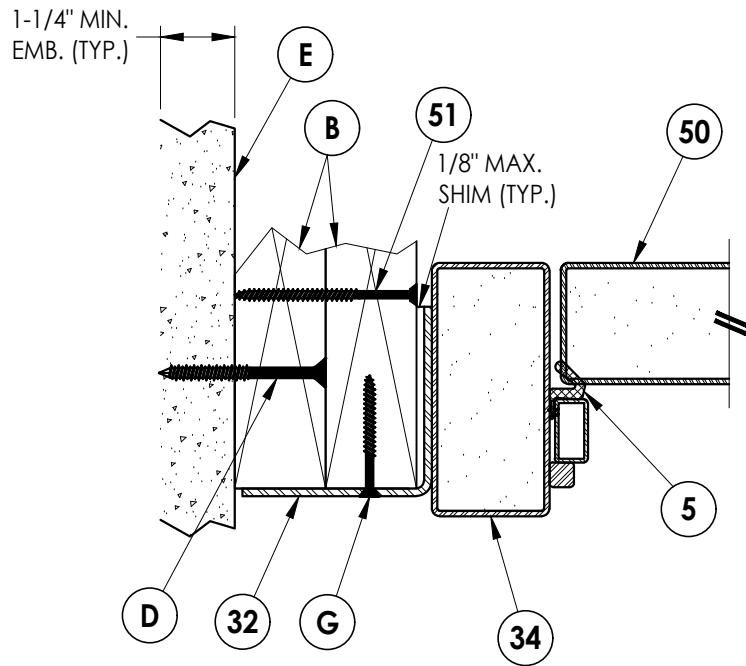
1 3 HORIZONTAL CROSS SECTION Outswing shown - inswing also approved
