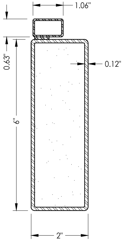
18 TOP, BOTTOM RAIL Foam filled
