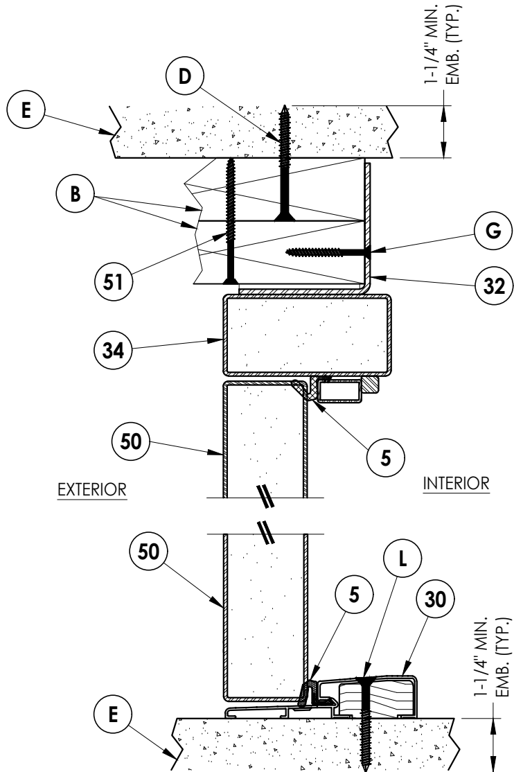
2 3 VERTICAL CROSS SECTION Outswing shown - inswing also approved
