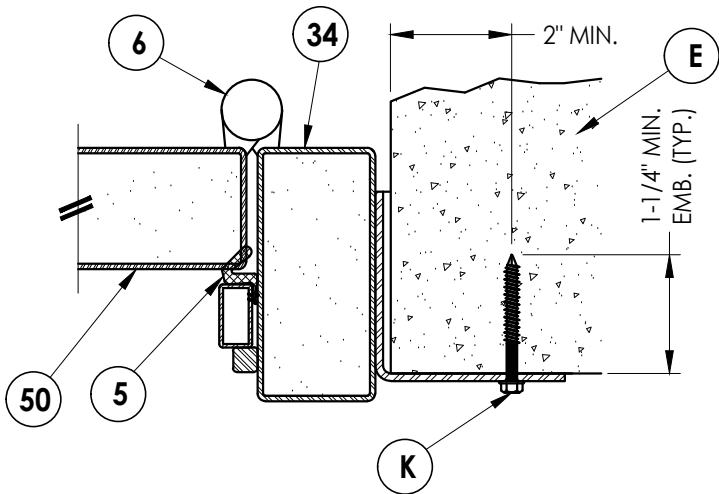
3 3 HORIZONTAL CROSS SECTION Direct to masonry
